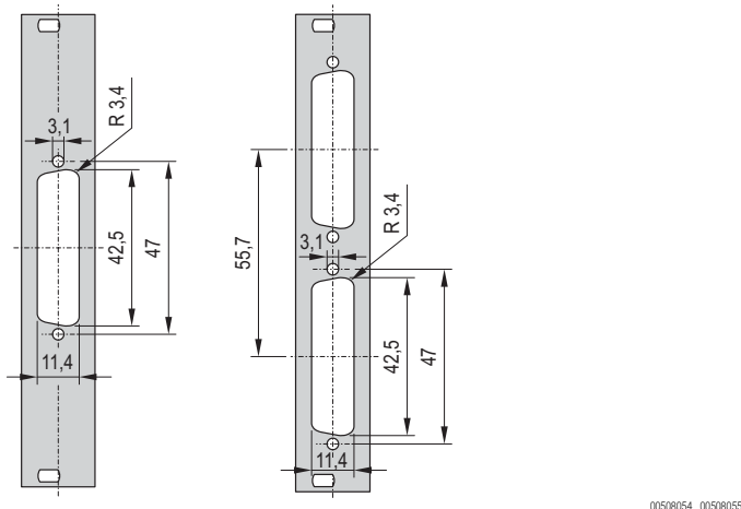
Frontplatte Sub-D 25-polig
