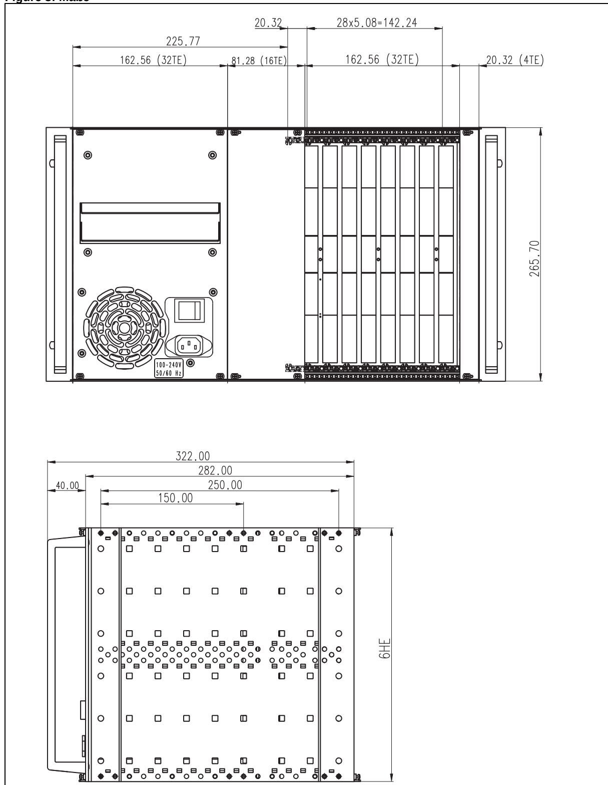
Figure 3: Maße
