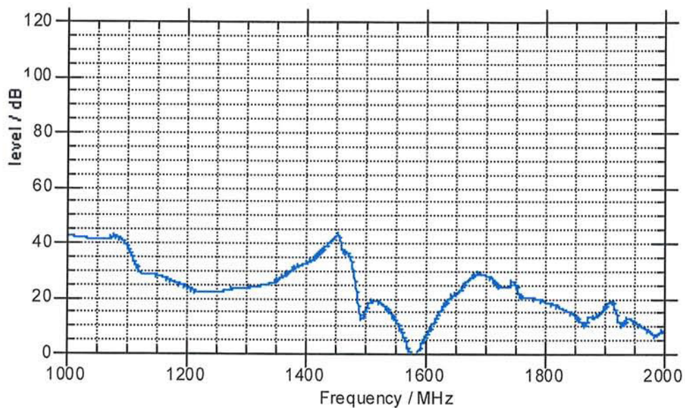
Fig. 6: Typical shielding effectiveness and worst case scenario of the EUT
